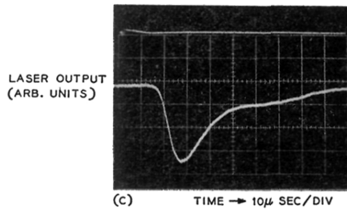
FIG. 3. Behavior of the CO 2 laser at 10.6324 μ under pulsed discharge conditions; (a) top trace: pulse voltage (15-kV peak); middle trace: pulse current (15-A peak); bottom trace: 4830-Å light output (CO B 1 Σ → A 1 Π band) from the side of discharge tube. Time scale = 1 μ sec/division for all three traces. (b) top trace: laser output at 10.6324 μ; middle trace: 4830-Å light output from the side; bottom trace: current pulse at far left. [Note the long (~300 μ sec) time delay between the current pulse and the commencement of laser oscillation.] Time scale: 50 μ sec/division for both; (c) laser output display on a 10-μ sec/division time scale showing long decay time.
