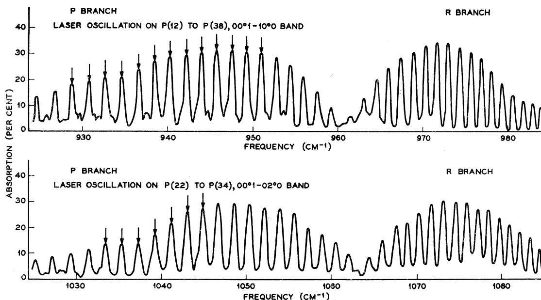
FIG. 1. Absorption spectrum for (a) 00°1-10°0 band (top) and (b) for 00°1-02°0 band (bottom) as measured by Barker and Adel in Ref. 1. The frequency scale is corrected in both the cases to read vacuum wave numbers. The laser wavelengths are indicated by arrows on the particular transitions responsible.
